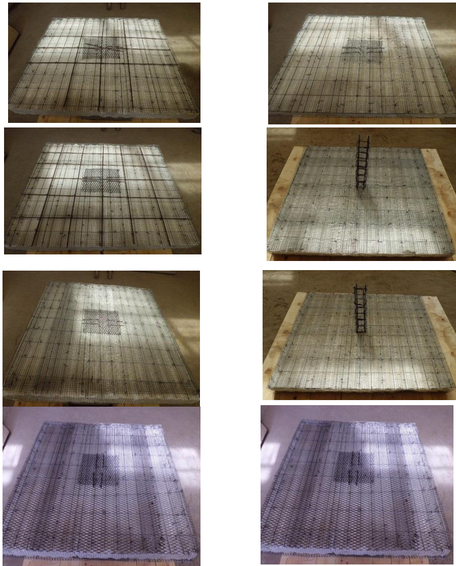
Figure 9: Reinforcement configuration of all tested light weight slabs
