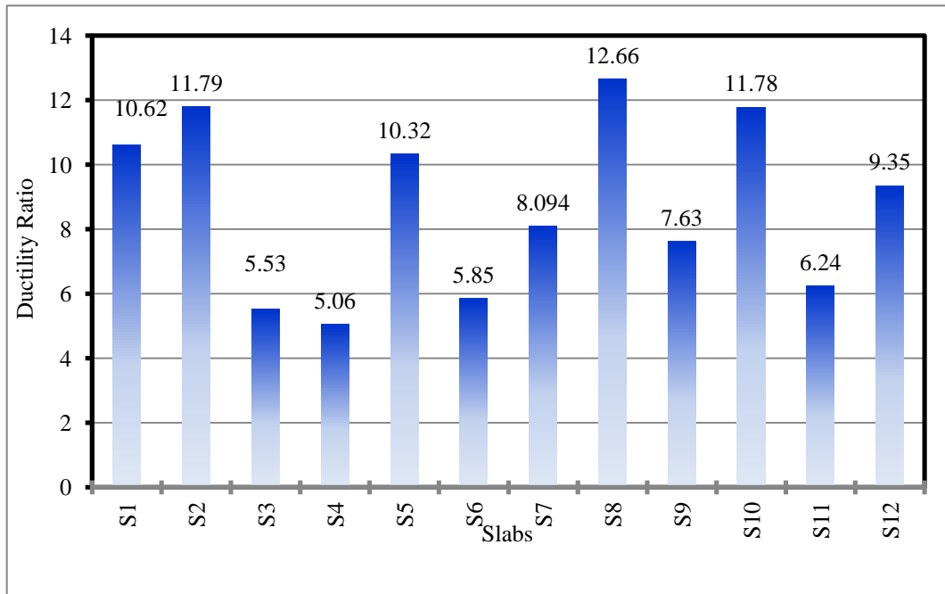
Figure 7: Ductility Ratio for all Slabs
