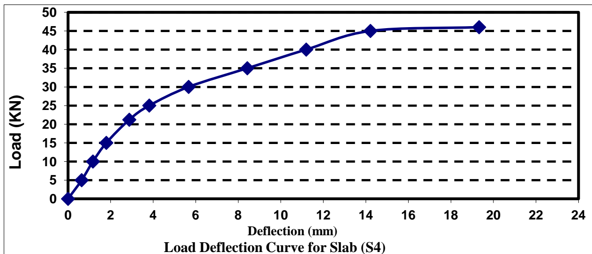
Figure 3: Load central deflection of slabs S1-S4
