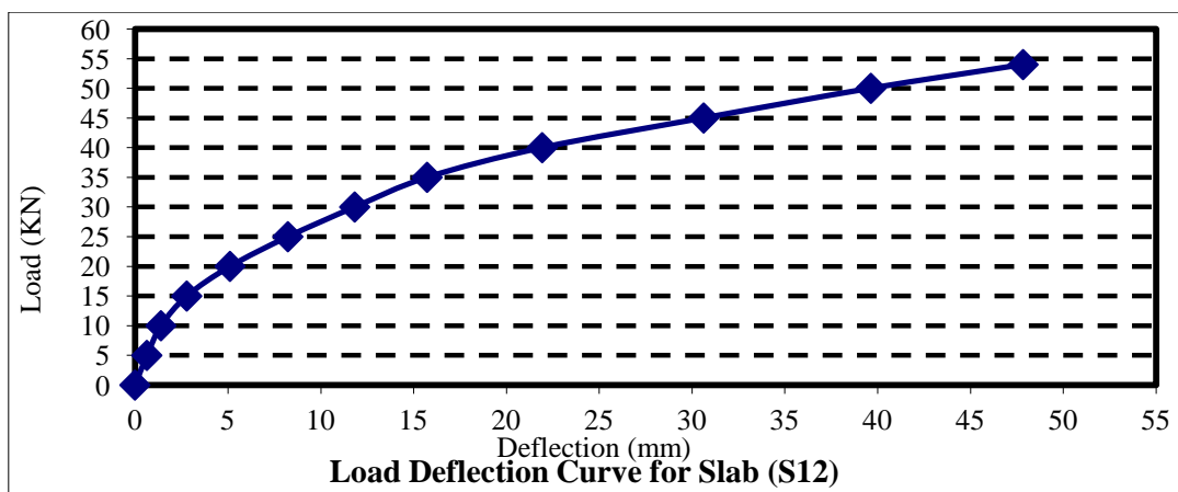
Figure 5: Load central deflection of slabs S4-S12
