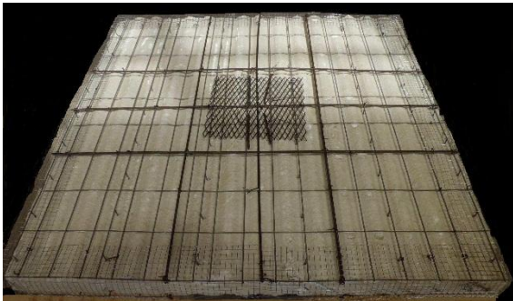
Figure 1: Lightweight polystyrene block panel
