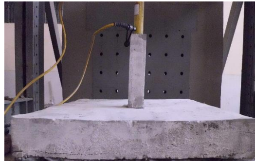
Figure 2: Test Rig 1200x1200mm and 80mm thick
