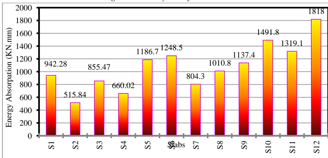
Figure 8: Energy Absorption for all Slabs
