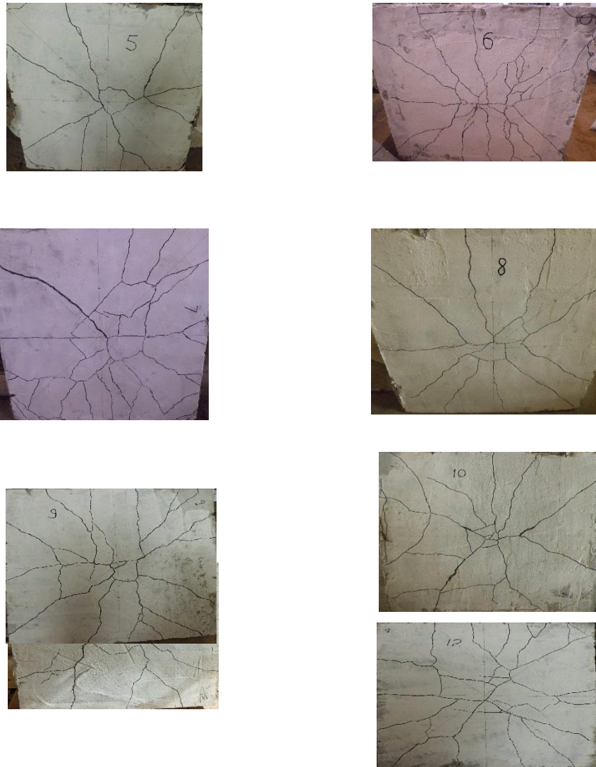
Figure 10: Cracking patterns in the tension face of all the tested slabs
