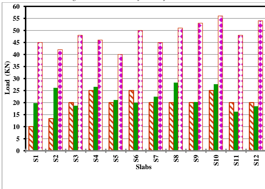
Figure 6: Comparison of First Crack & Serviceability and Ultimate Load for all Slabs
