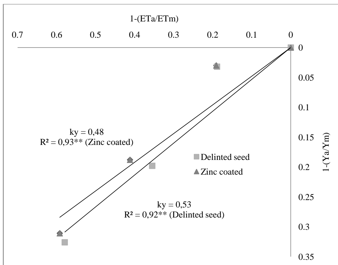
Figure 2: Yield response factor, k_y , cotton seed applications
