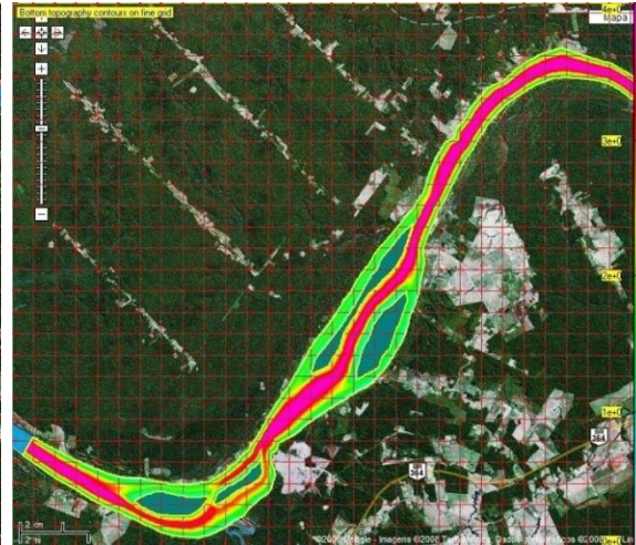
Figure 5: Bottom topography
