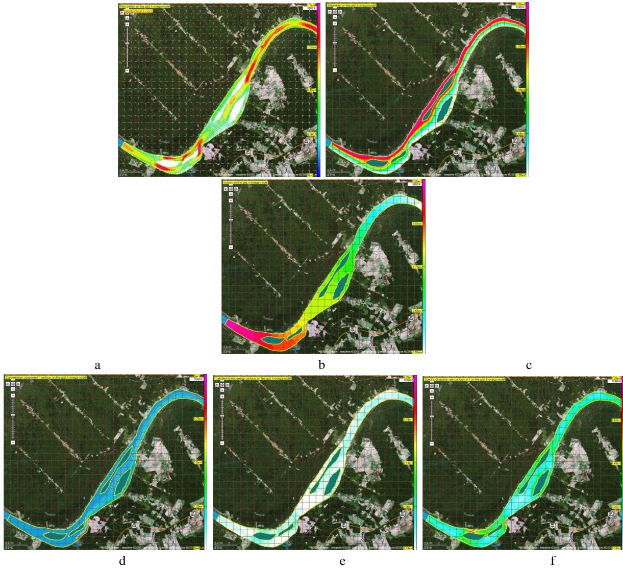
Figure 6: A part of results, calculated by \tilde{k} - \tilde{\omega} model
