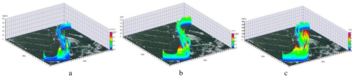
Figure 7: 3D \tilde{k} distributions, calculated by \tilde{k} - \tilde{\omega} , \tilde{k} - \tilde{\epsilon} and \tilde{k} - \tilde{w} models
