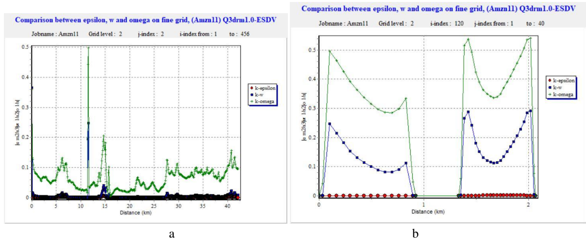
Figure 12: \tilde{\omega} , \tilde{\epsilon} and \tilde{w} at a: i from 1 to 456 and j=2 ; b: i=120 and j from 1 to 40
