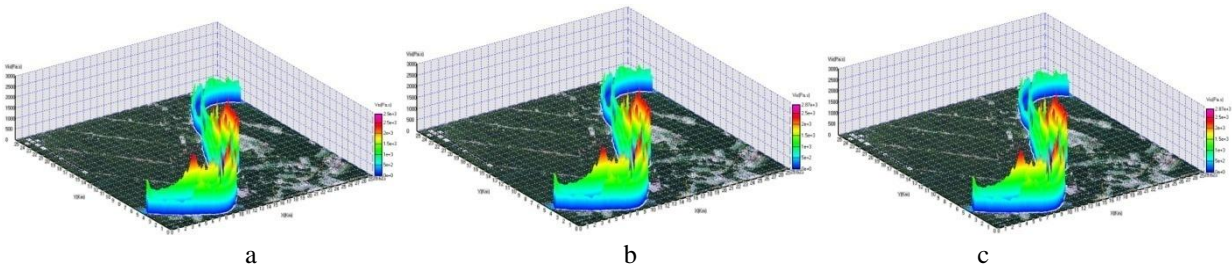
Figure 9: 3D \tilde{\mu}_{eff} distributions, calculated by \tilde{k} - \tilde{\omega} , \tilde{k} - \tilde{\epsilon} and \tilde{k} - \tilde{w} models
