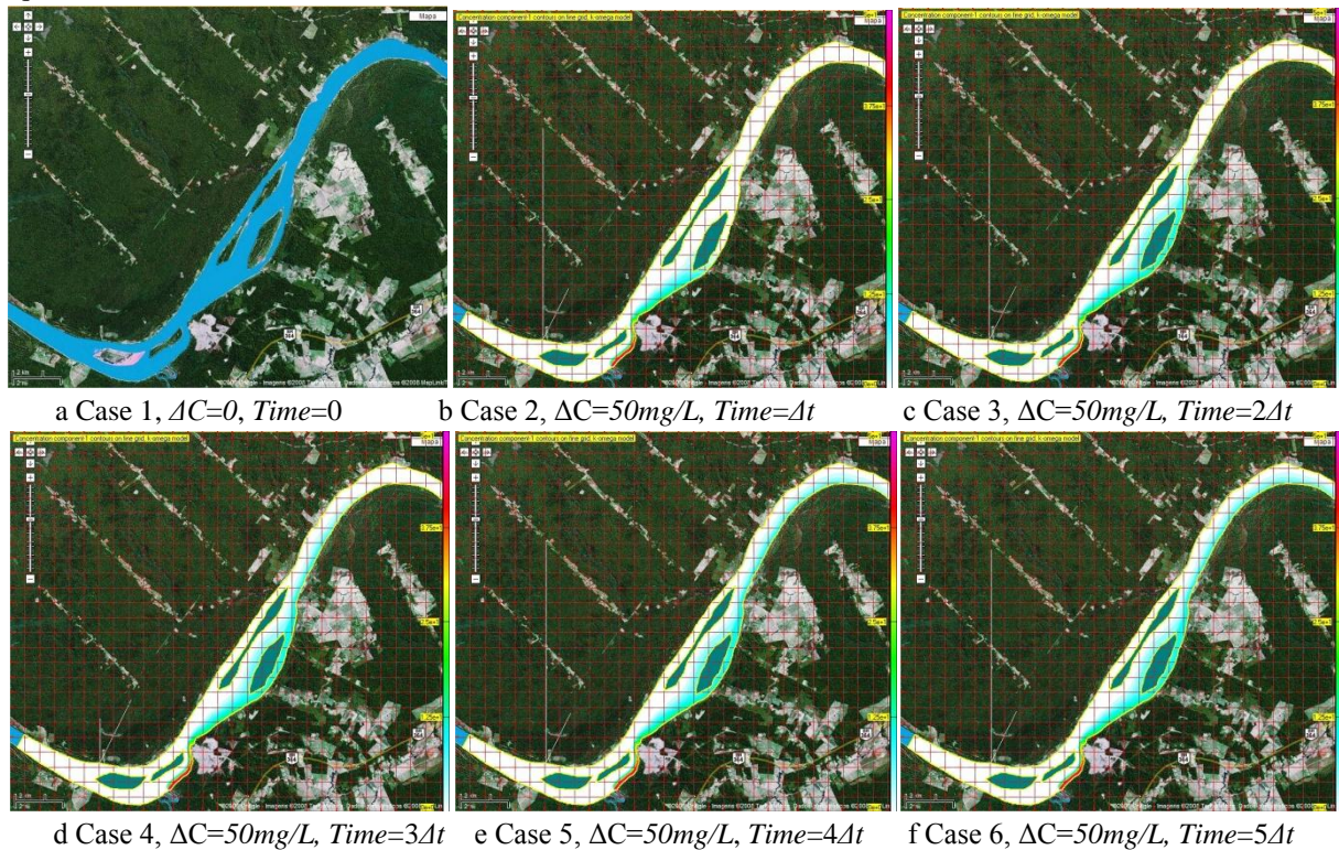
Figure 13: Contaminant plume development
