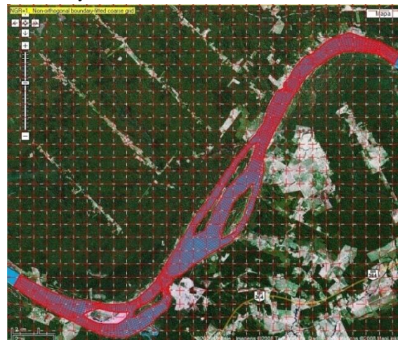
Figure 3: Coarse grid
