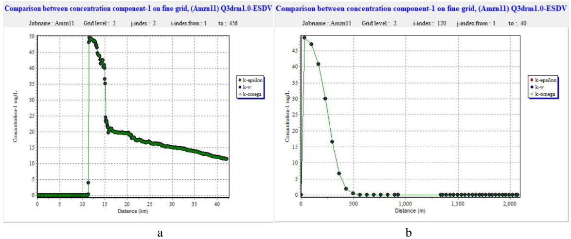
Figure 11: Concentrations at a: i from 1 to 456 and j=2 ; b: i=120 and j from 1 to 40
