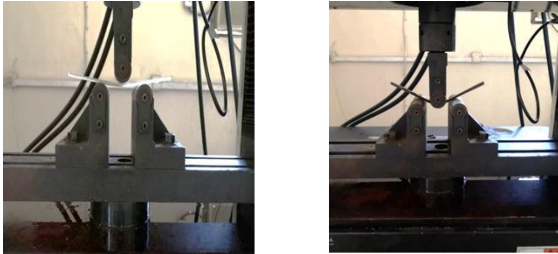
Figure 1: Concrete Flexural Machine
