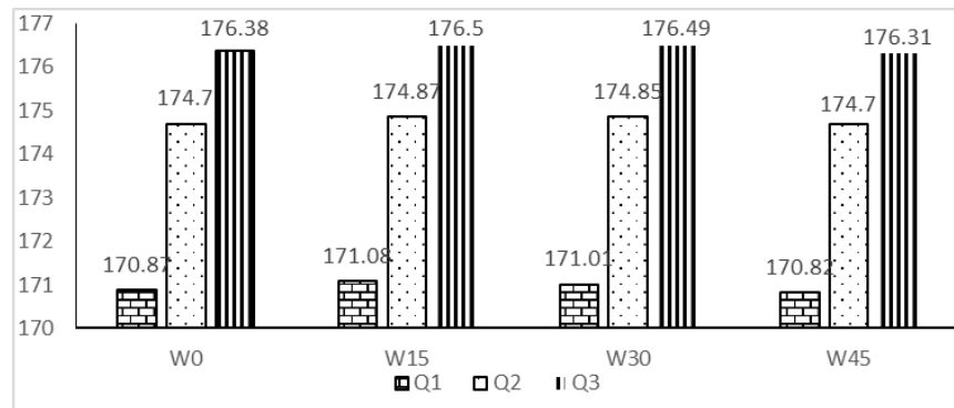
Figure 10: The weight loss ( \Delta M %) studied samples over 45 cycles of salt weathering
