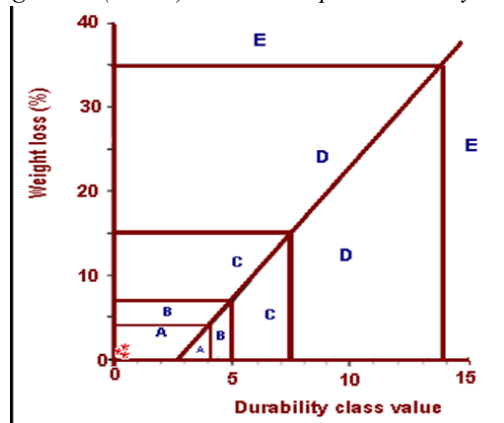
Figure 11: Barry diagram presenting durability class and value based on weight loss percentage of the studied samples
