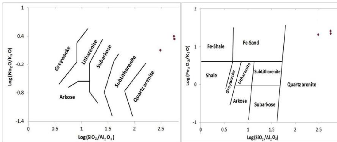
Figure 7: Geochemical classification of the studied quartzitic sandstone samples.
