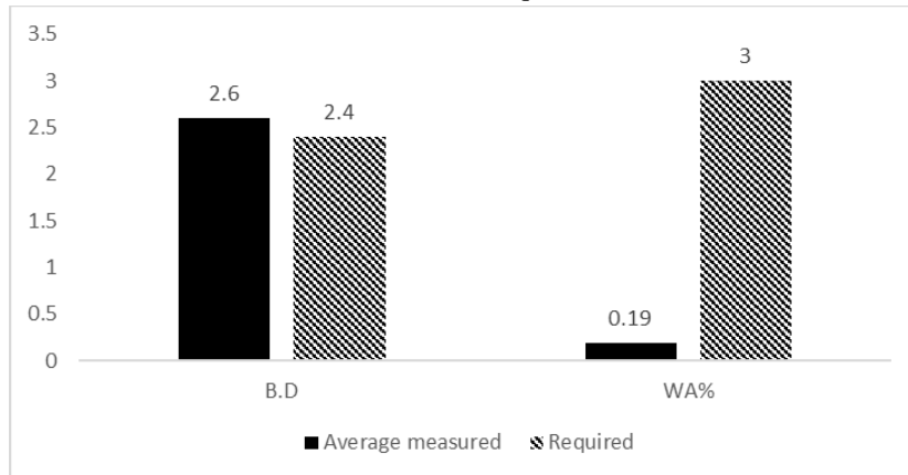
Figure 8: The comparison between measured and required average values of studied physical properties based on standard specification
