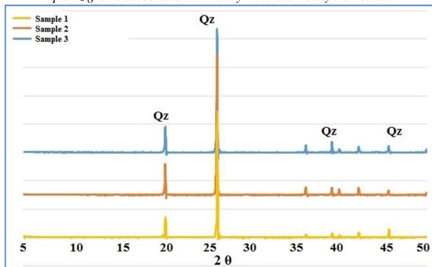
Figure 6: XRD pattern of studied samples
