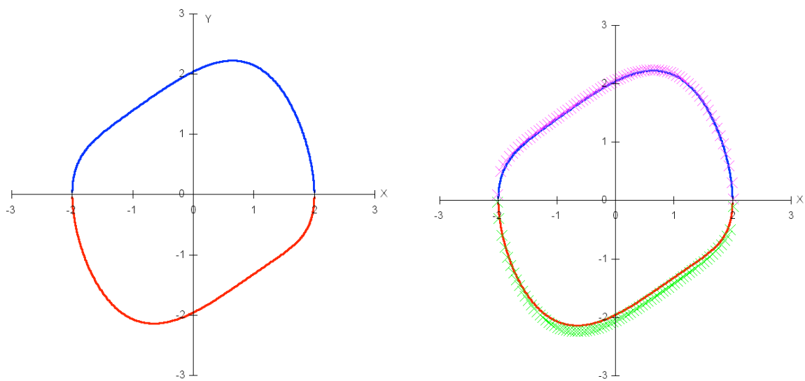
Figure 4: a) Analytic solution of the integral curve at order n = 2 when |A|=2, \varepsilon = .5 b)
