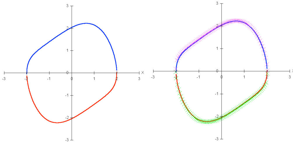
Figure 6: a) Analytic solution of the integral curve at order n = 3 when |A| = 2, \epsilon = .5 b) Comparison of the 3 rd order analytic result with Runge-Kutta method
