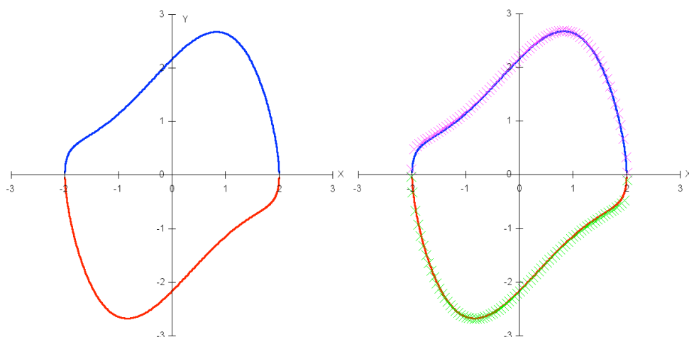
Figure 5: a) Analytic solution of the integral curve at order n = 2 when |A|=2, \varepsilon = 1
