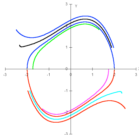
Figure 3: Analytic solutions of the integral curves at order n = 1 when A = |2|, \varepsilon = .5 (limit cycle) and branches of the phase trajectories in correspondence to |A| = 2.8, 2.4, 1.7365, C = .58, -1.3, -3 (from top to bottom)
