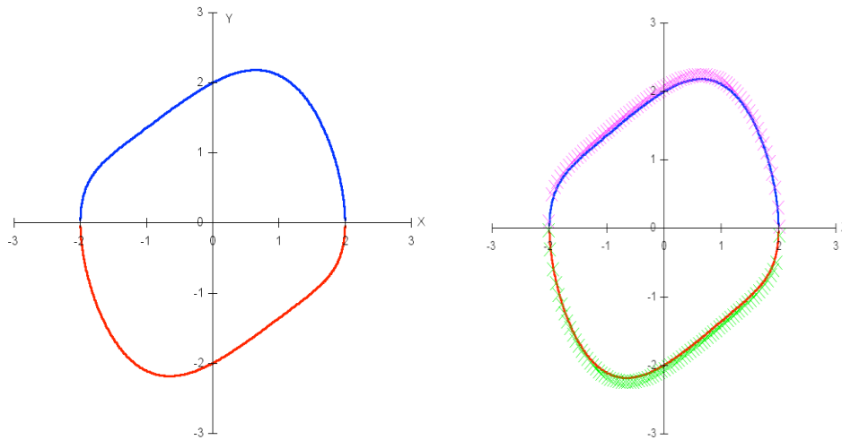
Figure 2: a) Analytic solution of the integral curve at order n = 1 when |A| = 2, \varepsilon = .5 ; b) Comparison of the 1 st order analytic result with Runge-Kutta method
