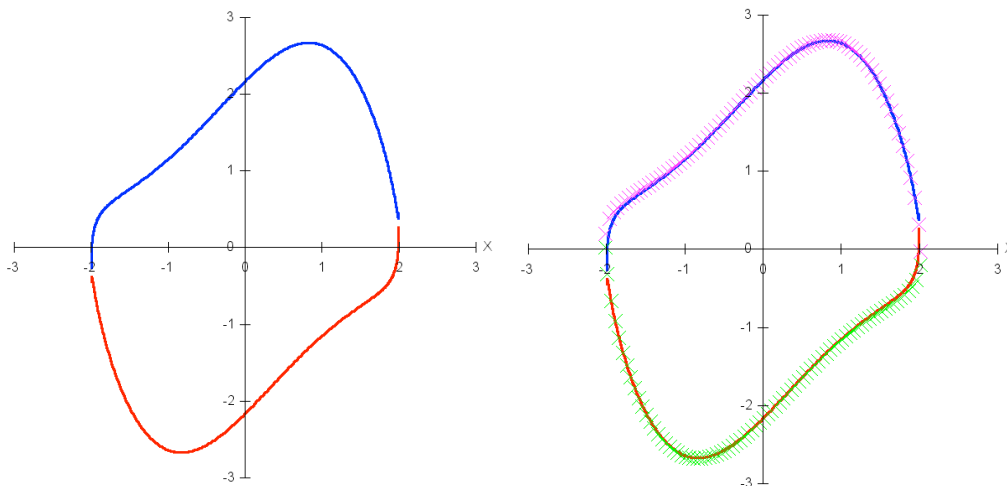
Figure 7: a) Analytic solution of the integral curve at order n = 3 when |A| = 2, \epsilon = 1 b) Comparison of the 3 rd order analytic result with Runge-Kutta method
