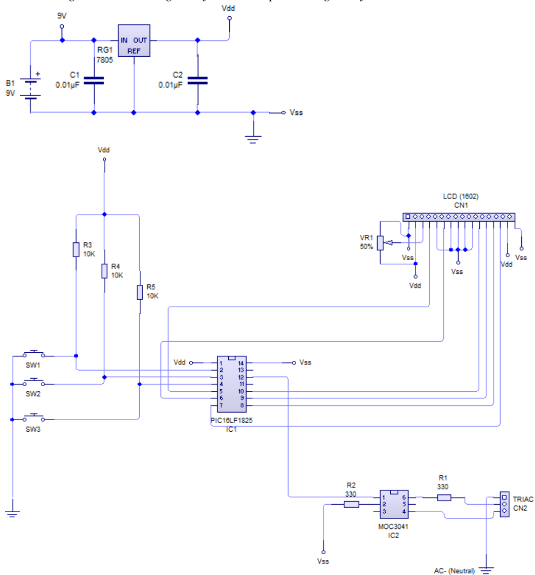
Figure 2: Circuit Diagram of the Developed Timing Unit for Electric Ovens
