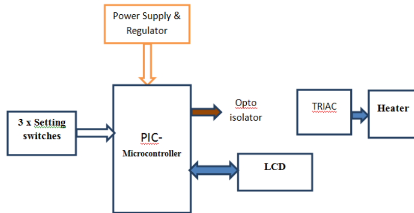
Figure 1: Block Diagram of the Developed Timing Unit for Electric Ovens
