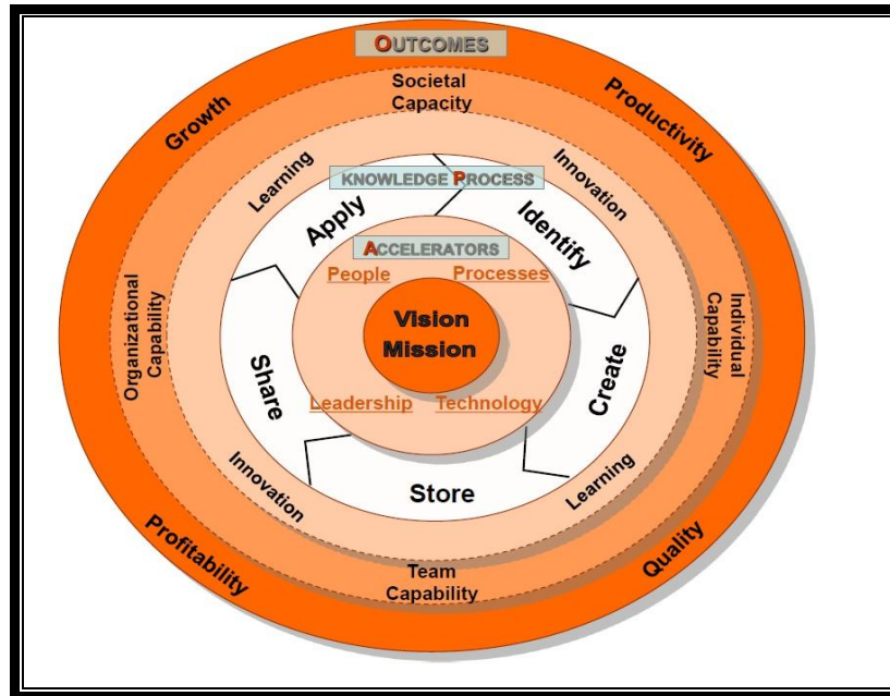
Figure 1: KM framework
