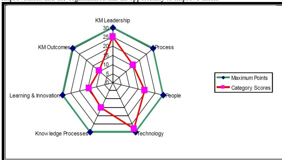
Figure 2: Radar Chart
